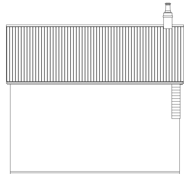
REAR ELEVATION
