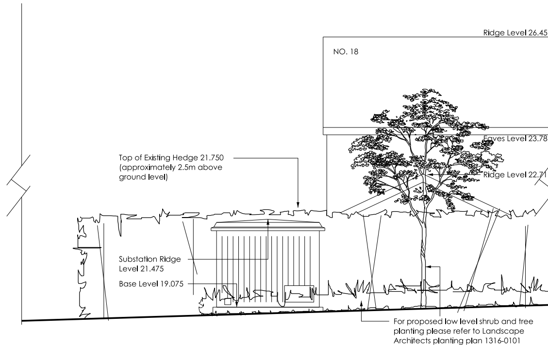
SUBSTATION SITE SECTIONAL ELEVATION
