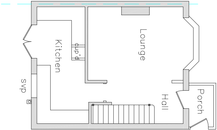
Ground Floor Layout
