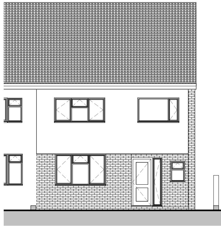
1 North Elevation 40 1 : 100
