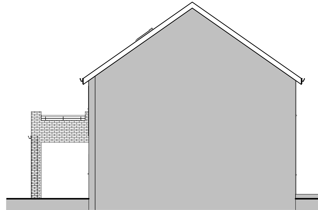
3 East Elevation/Section 40 1 : 100
