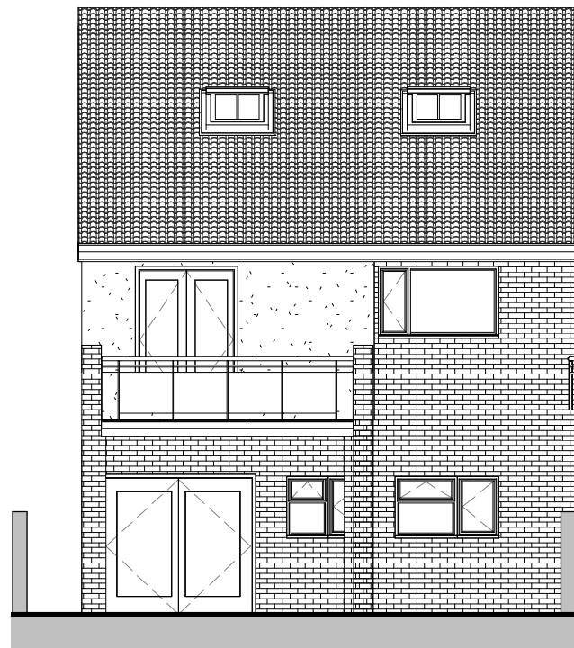
2 South Elevation 40 1 : 100
