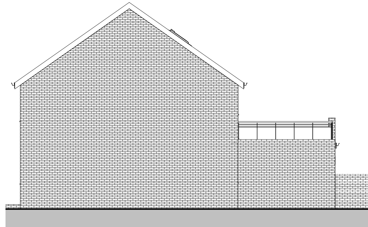
4 West Elevation 40 1 : 100
