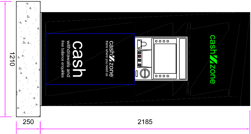
FRONT ELEVATION - BODEX POD w/NCR 6622e ATM
