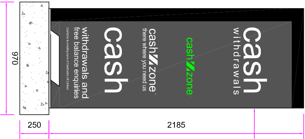
R/H/S ELEVATION - BODEX POD w/NCR 6622e ATM
