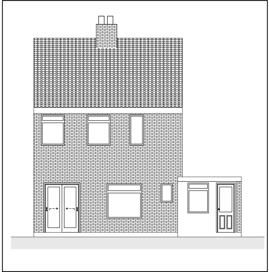
REAR ELEVATION
