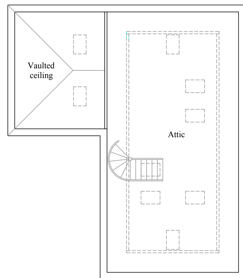
Attic Floor
