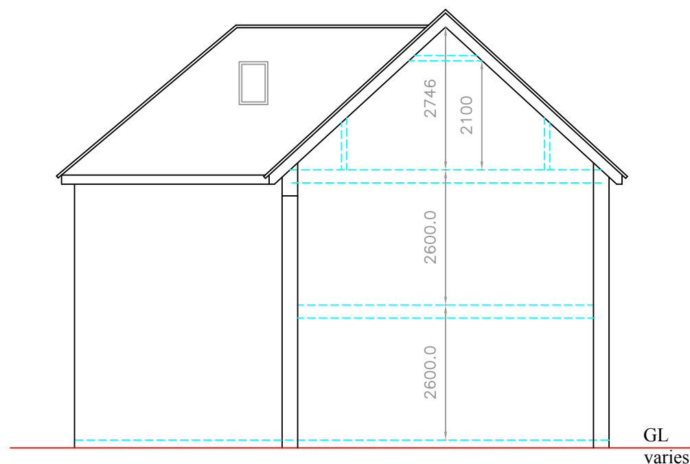
Draft Section
