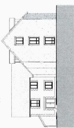
Apartments P- Left Elevation 1:200
