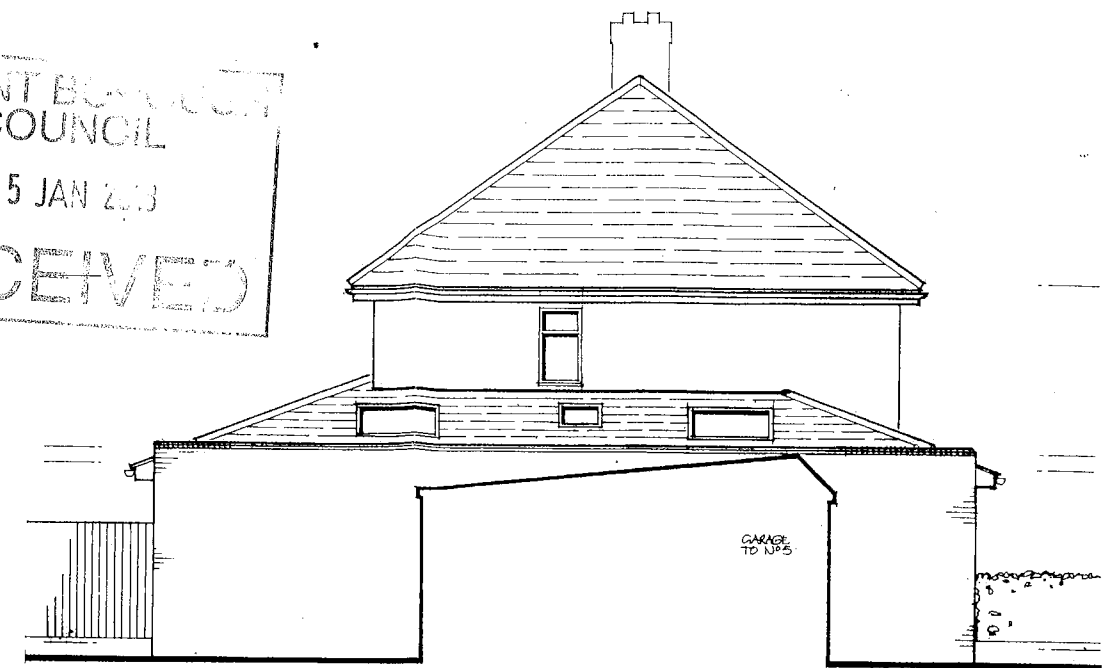
North Elevation
