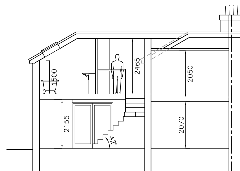
DRAFT SECTION
