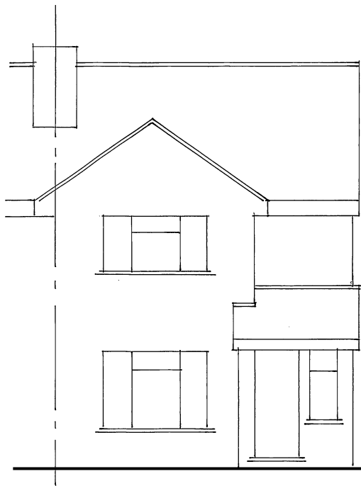
Existing East/Front Elevation
