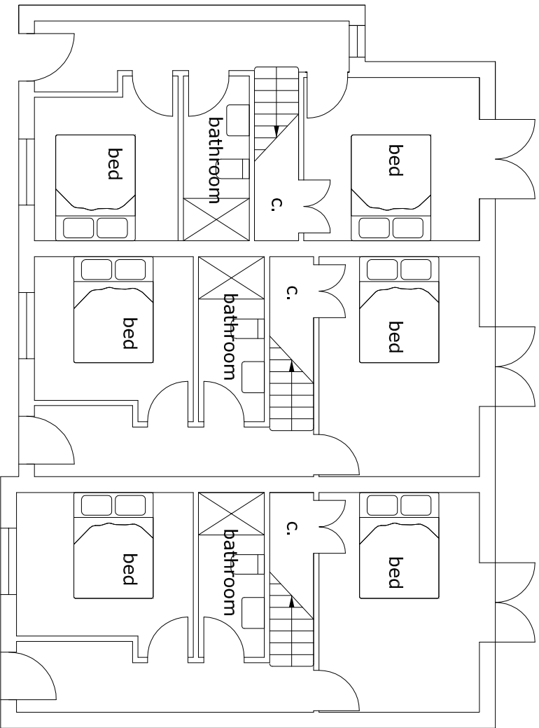
GROUND- PROPOSED 1:100
