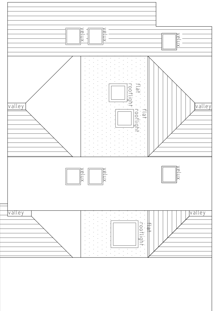
SECOND- PROPOSED 1:100
