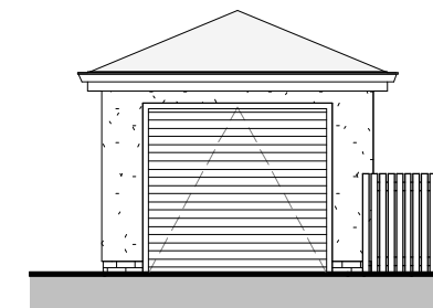
4 Front Garage Elevation 1 : 100
