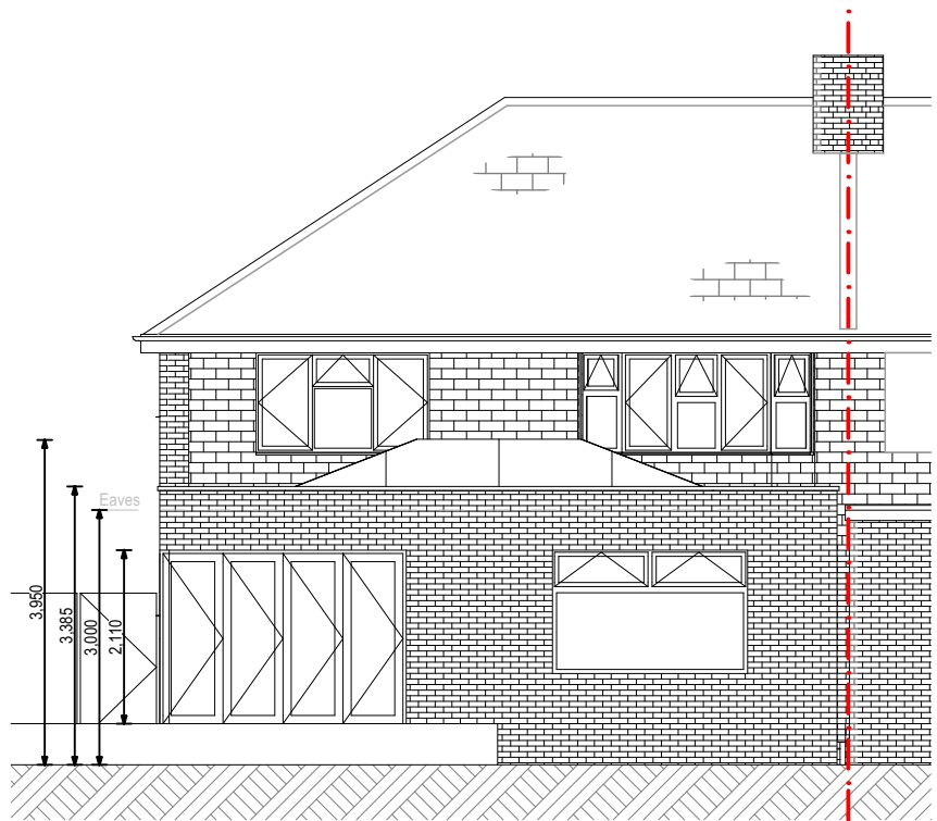
Elevation - Proposed
