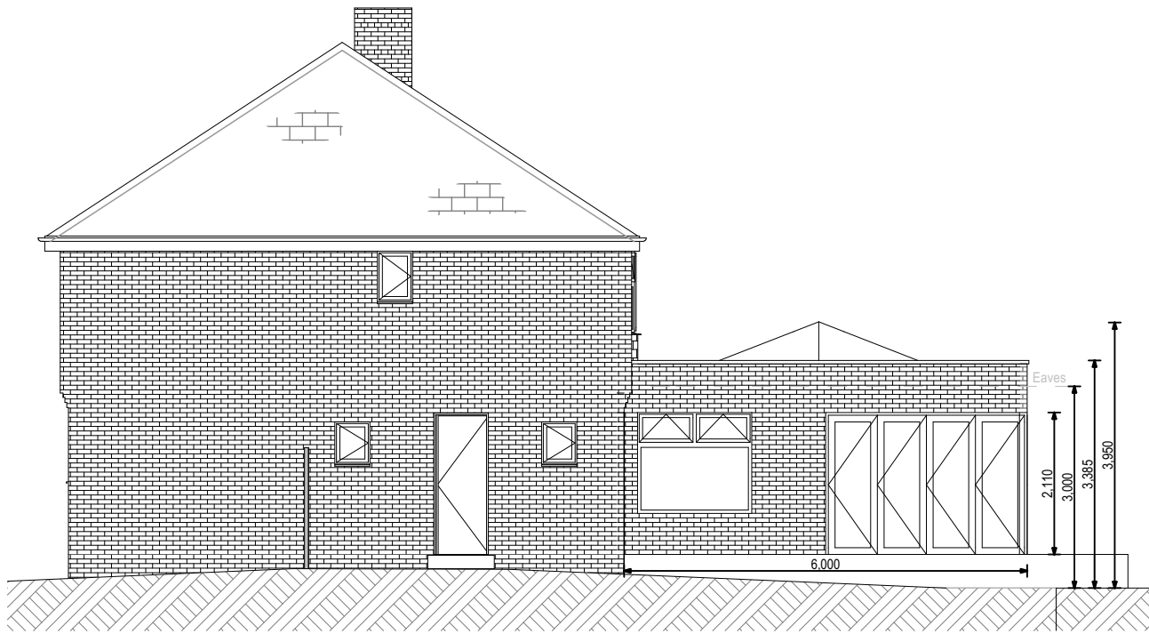
Elevation - Proposed
