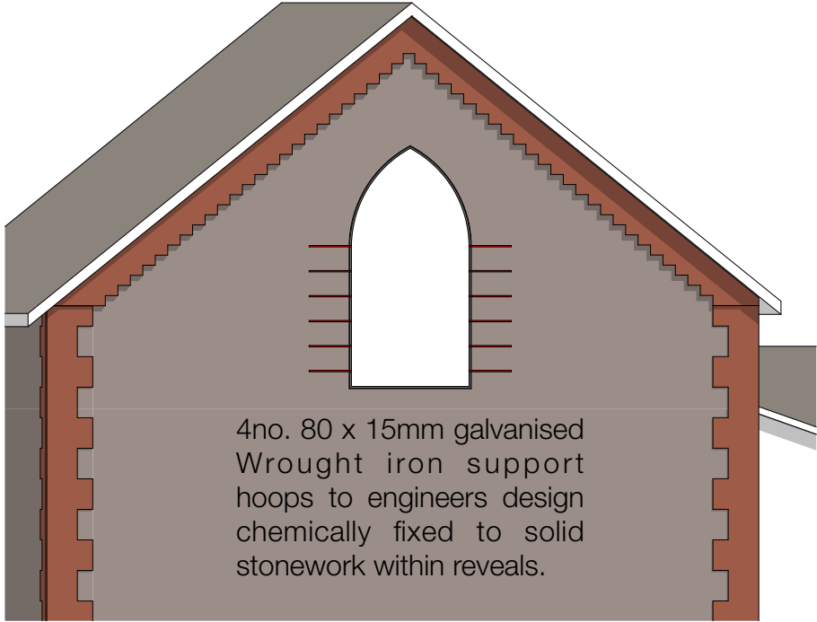
E-02 window stage 2 1:50
