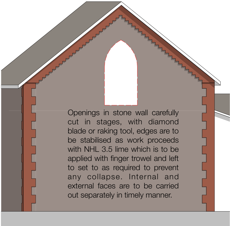
E-02 window stage 1 1:50
