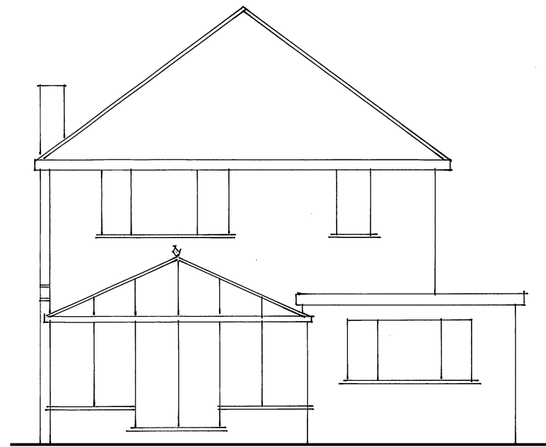
Existing NW/Rear Elevation
