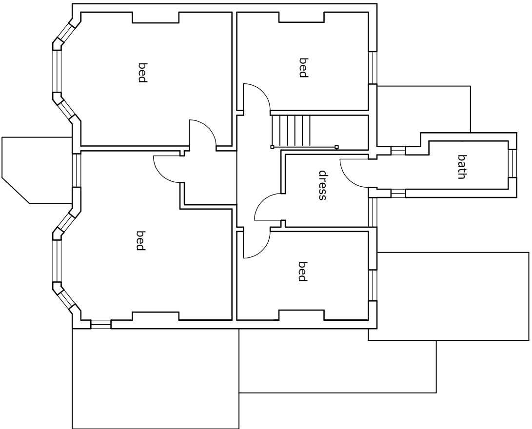
FIRST 1:100
