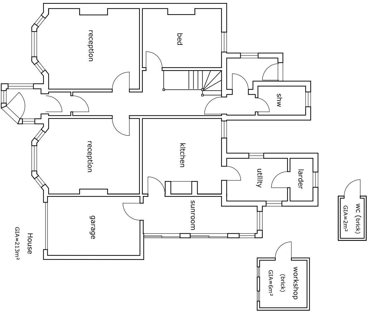
GROUND 1:100
