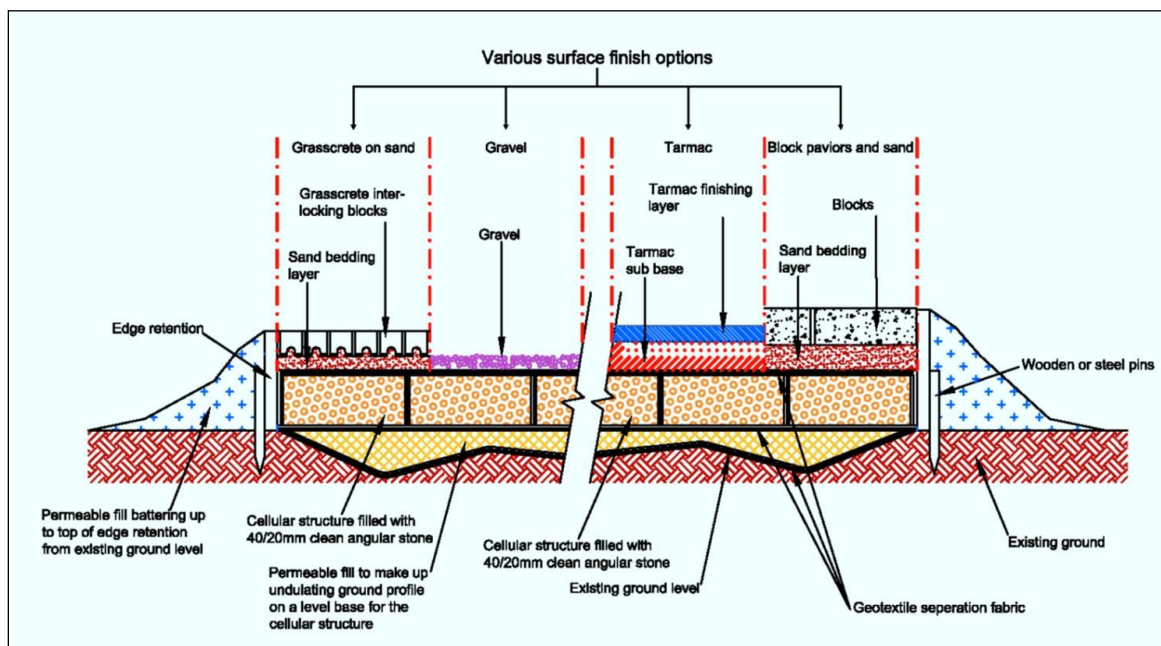
Figure 2: This conceptual cross-section illustrates the structural elements of the system and the multiple surfacing options that can be used with it.
