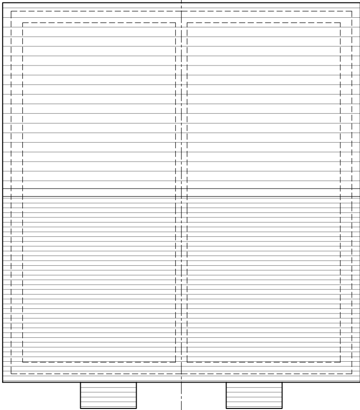
Roof Plan
