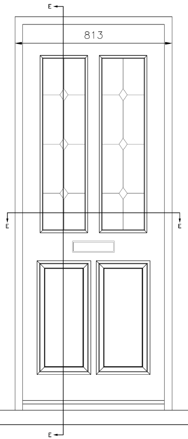
Section E Vertical
