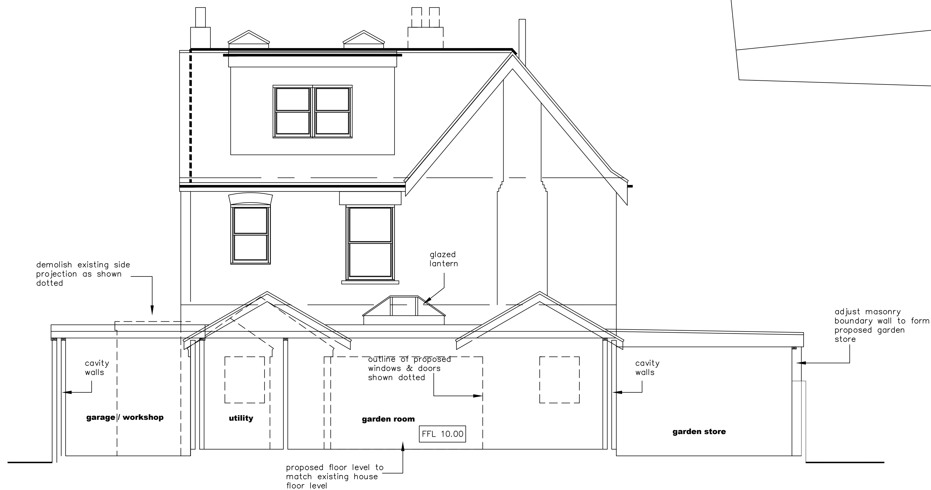
PROPOSED SECTION / SITE SECTION SCALE 1 : 50
