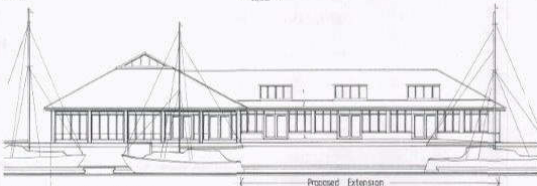
EAST (WATERFRONT) ELEVATION 1:300
