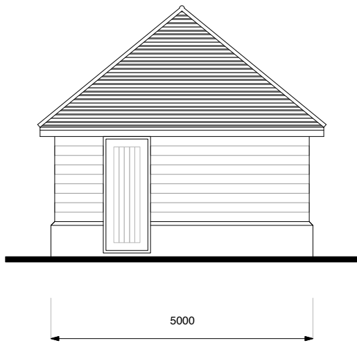
Existing SOUTH EAST (Side) Elevation at 1:100 scale
