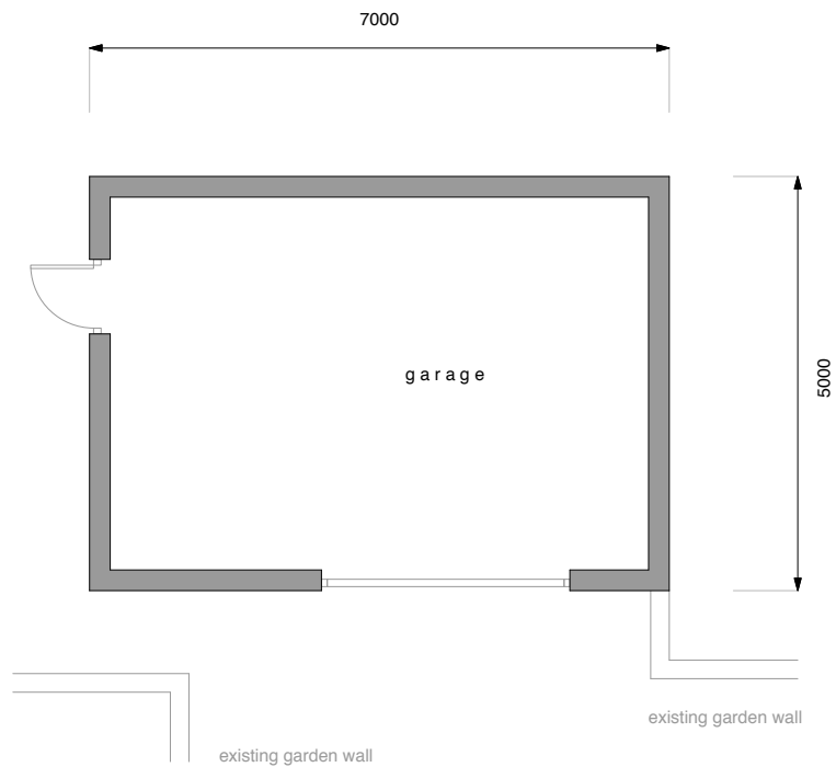
Existing Floor Plan at 1:100 scale
