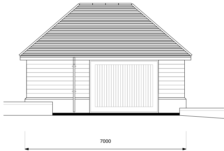
Existing NORTH EAST (Front) Elevation at 1:100 scale
