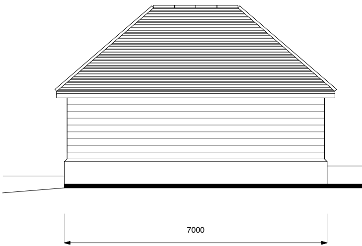
Existing SOUTH WEST (Rear) Elevation at 1:100 scale
