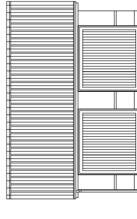
FRONT ELEVATION
