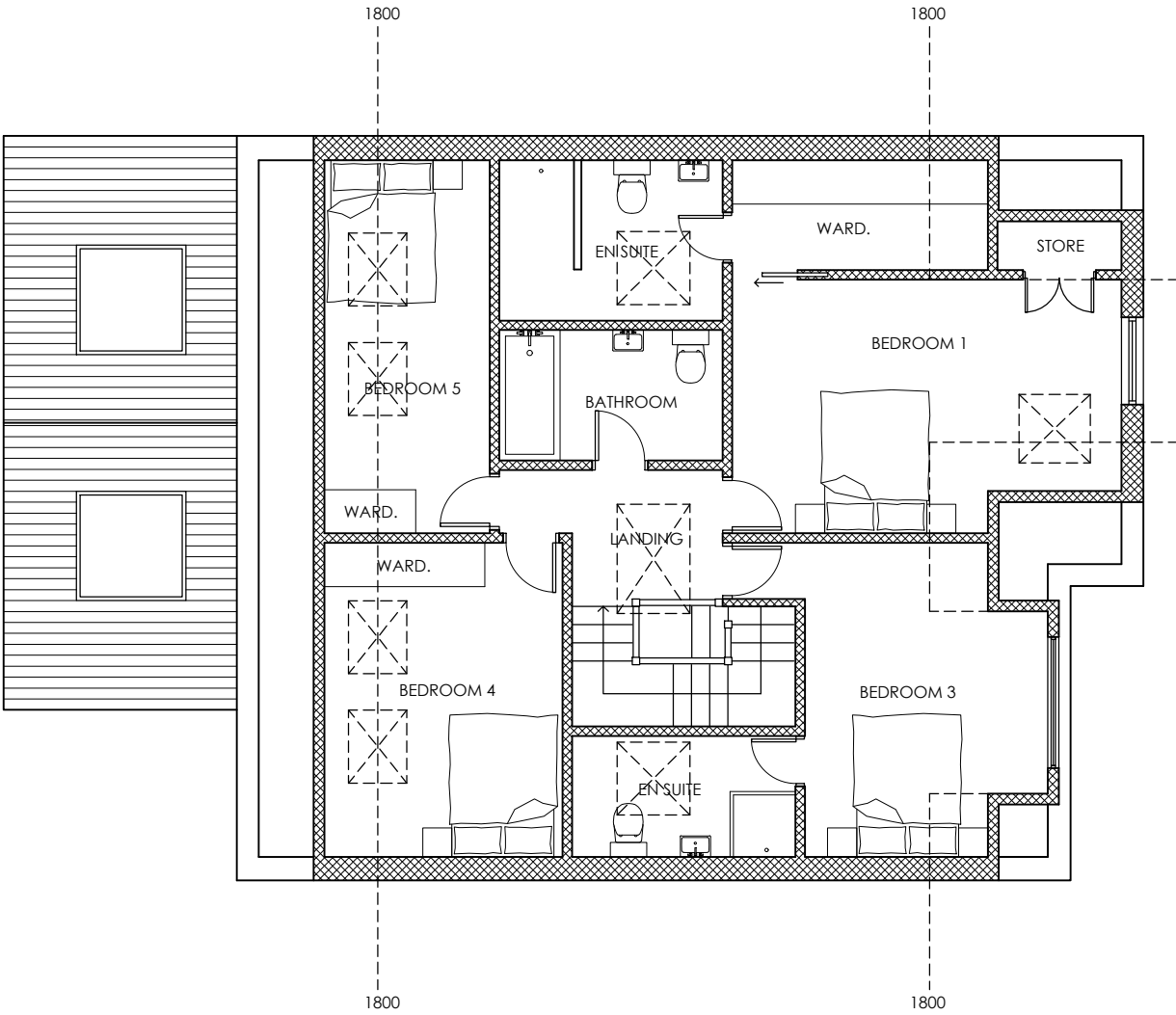
PROPOSED FIRST FLOOR PLAN OPTION 2A
