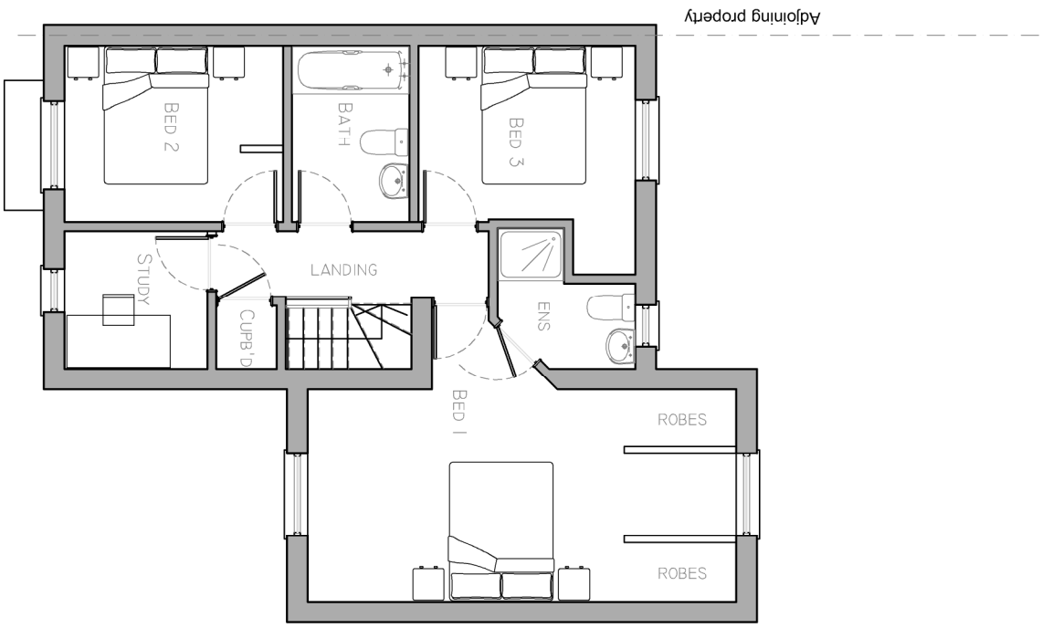
Existing First Floor Plan Scale 1:100
