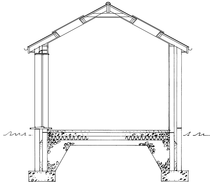
Cross-Section
