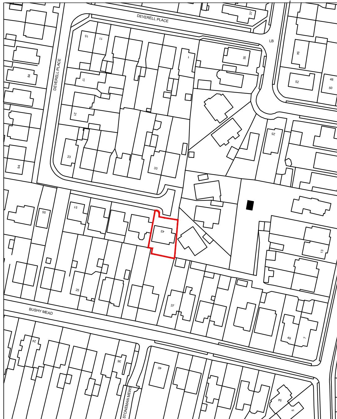
Location Plan: 1:1250
