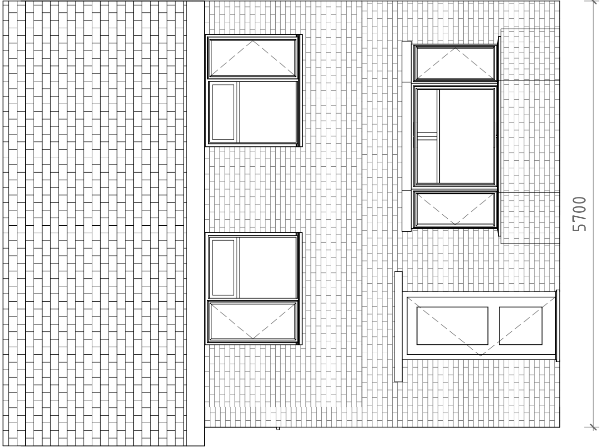
301 - EXISTING FRONT ELEVATION
