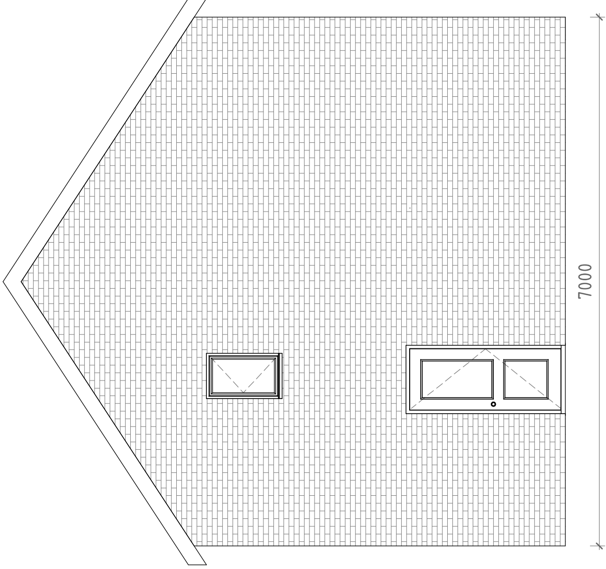
302 - EXISTING LEFT ELEVATION
