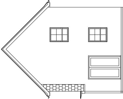
SIDE ELEVATION 2
