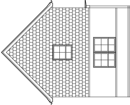
SIDE ELEVATION 1
