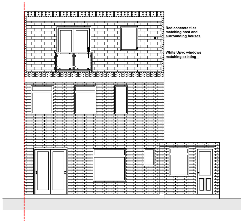
REAR ELEVATION
