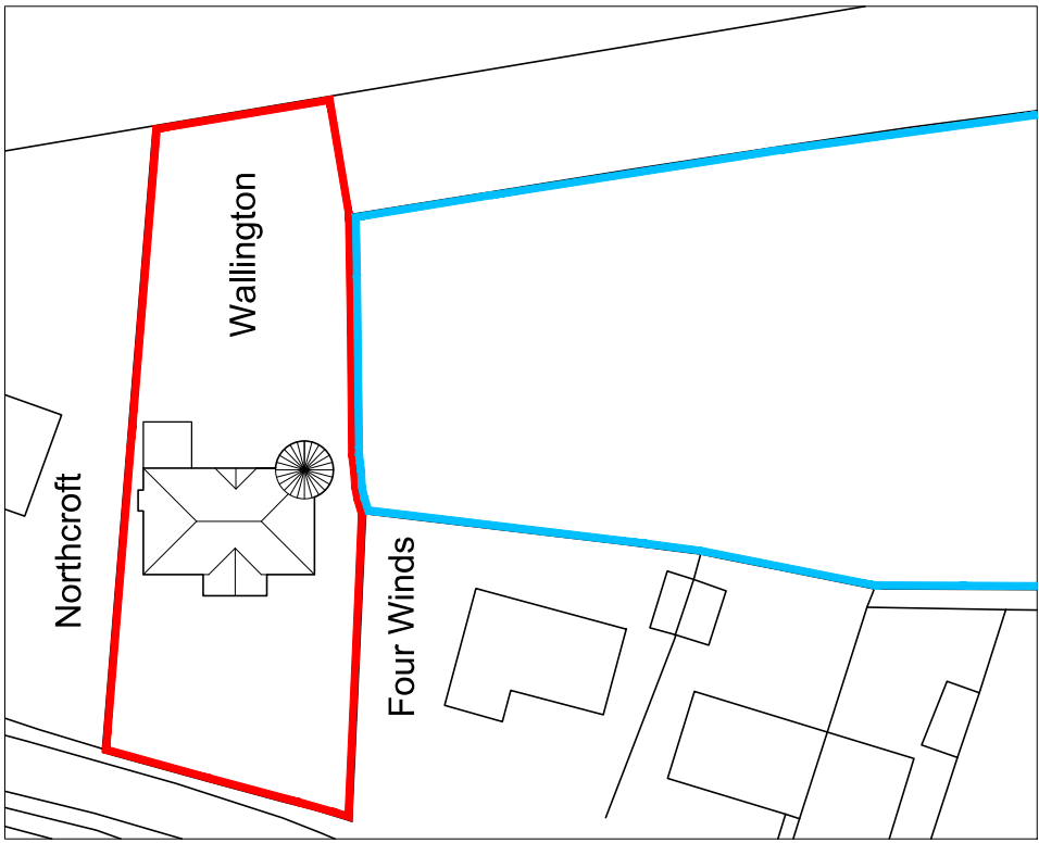
Block Plan: 1:500
