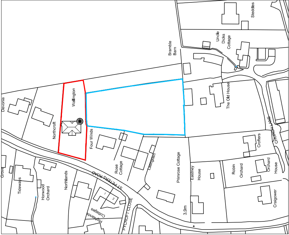
Location Plan: 1:1250
