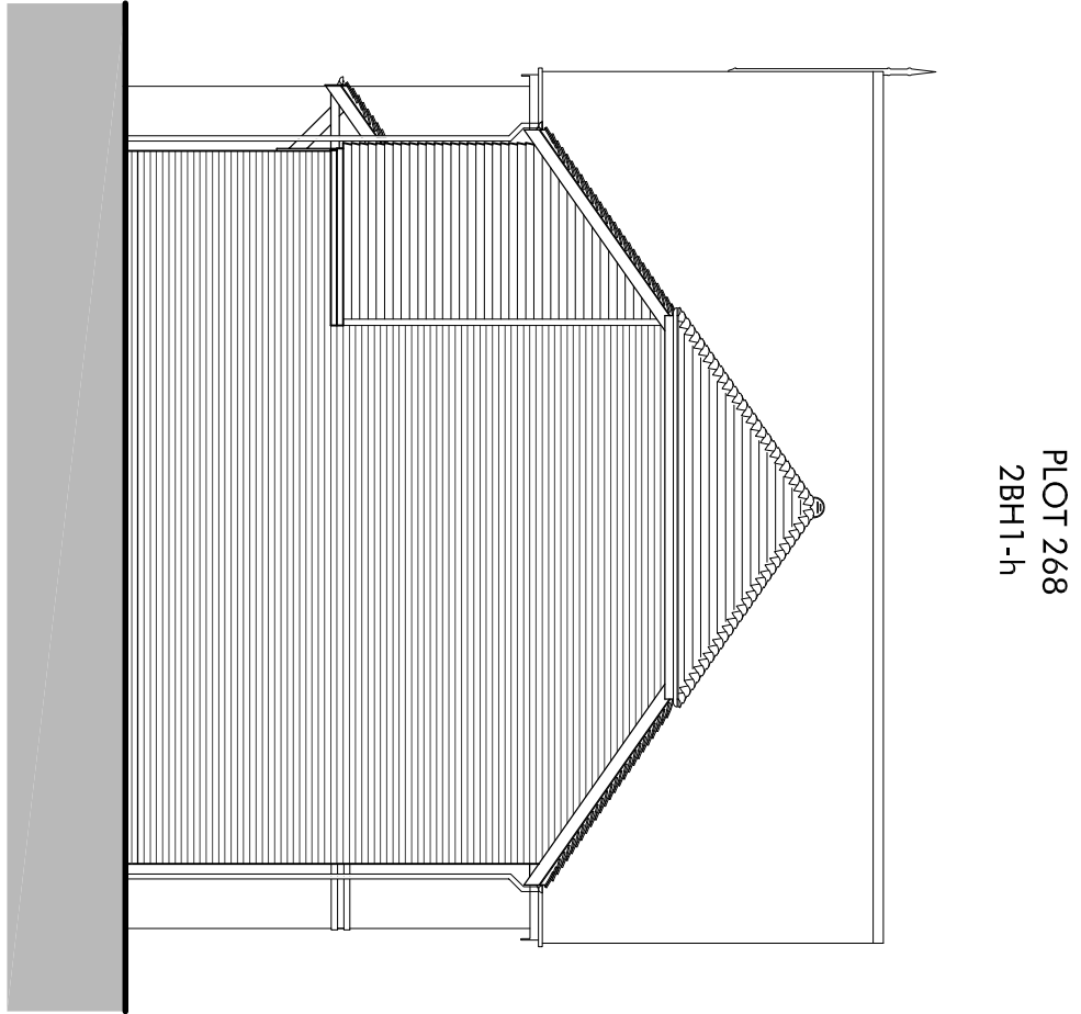
SIDE ELEVATION - B
