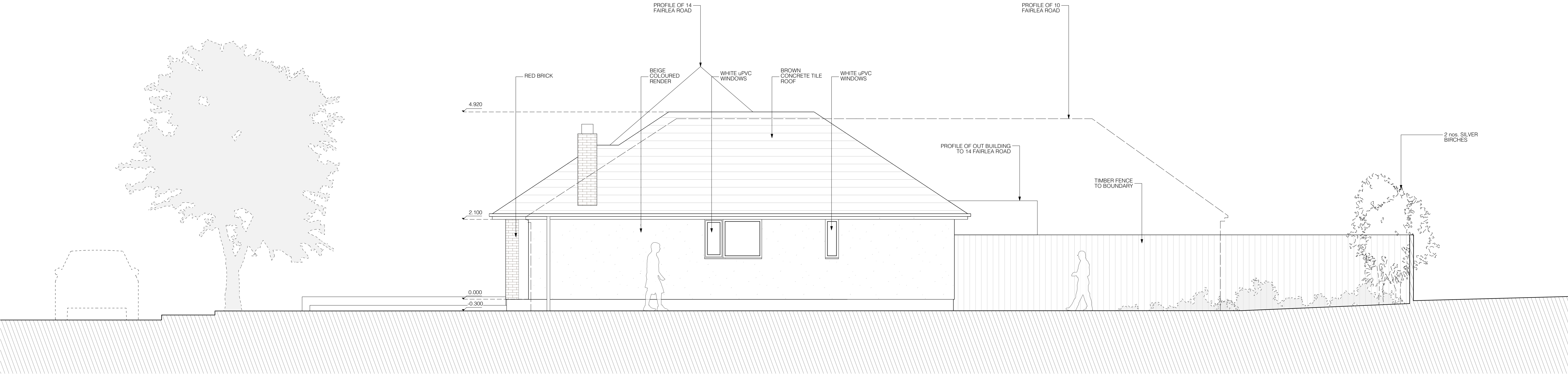
02 EXISTING EASTERN ELEVATION 1:50
