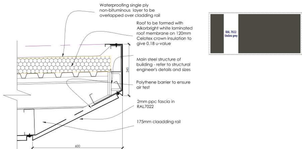
Fig 6 Roof capping detail (2mm PPC) - Ral 7022 – The proposed colour of the Roof capping
