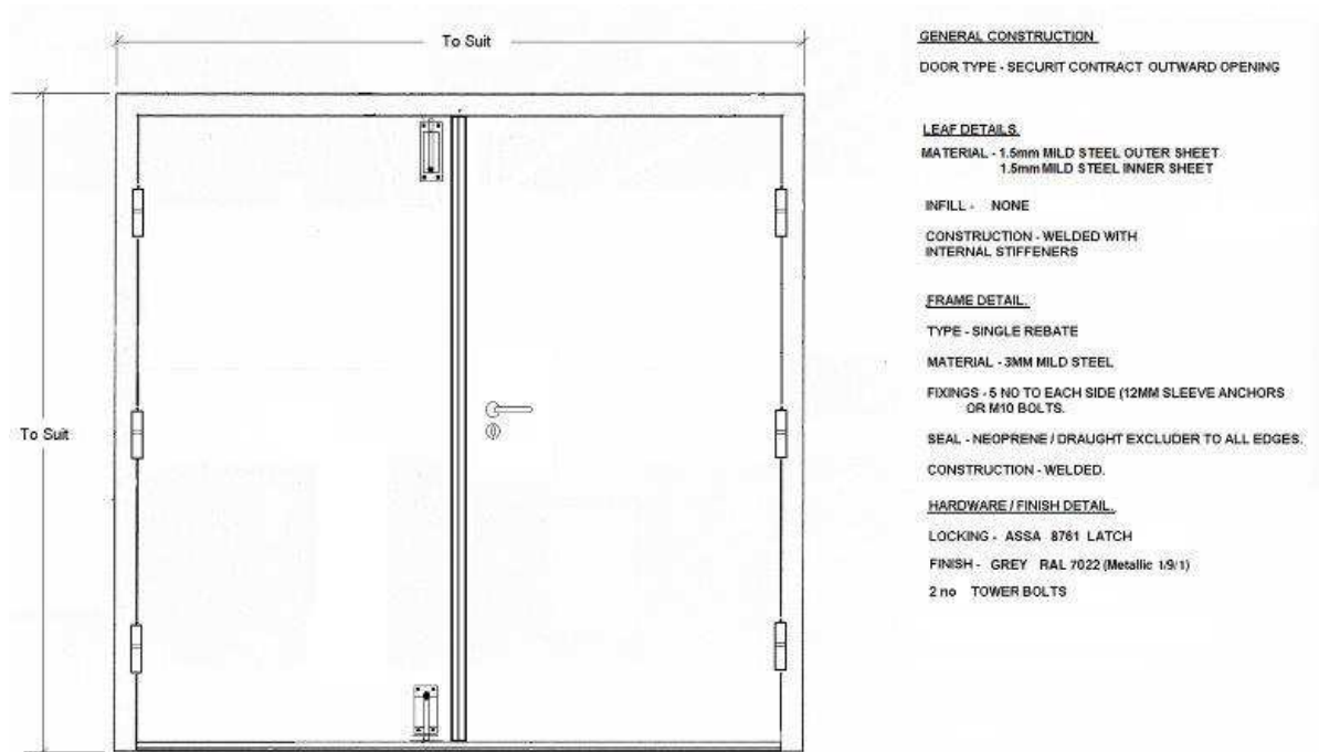
Fig 5 Soham Senator mild Steel security Yard door details and photographs
