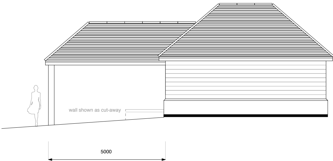
Proposed SOUTH WEST (Rear) Elevation at 1:100 scale
