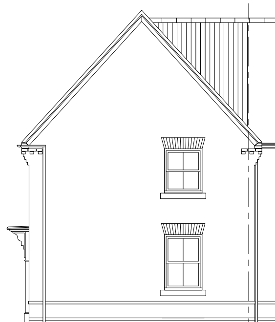
SIDE ELEVATION 1
