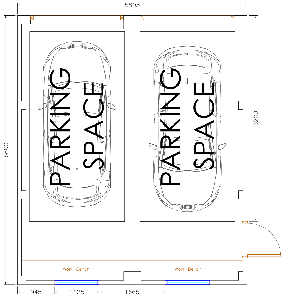
PROPOSED GARAGE FLOOR PLAN
