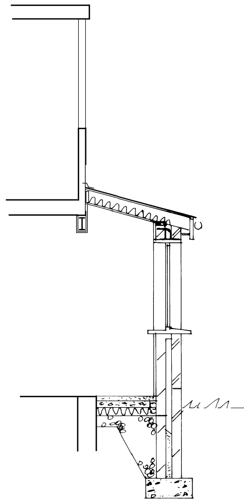
Cross-Section
