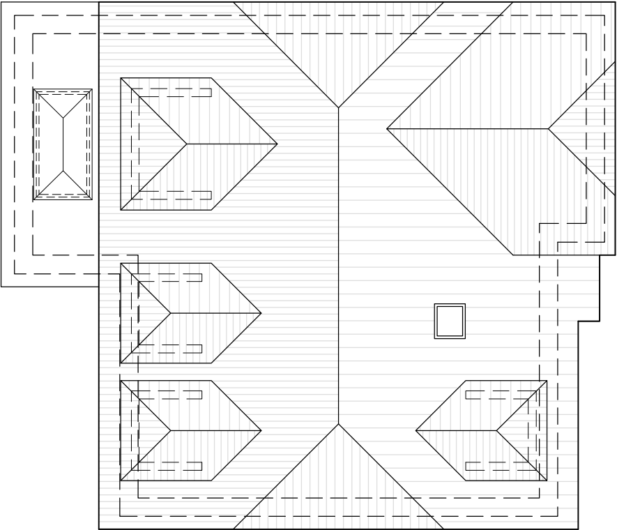
Roof Plan 1:100 Plots 3 & 4
