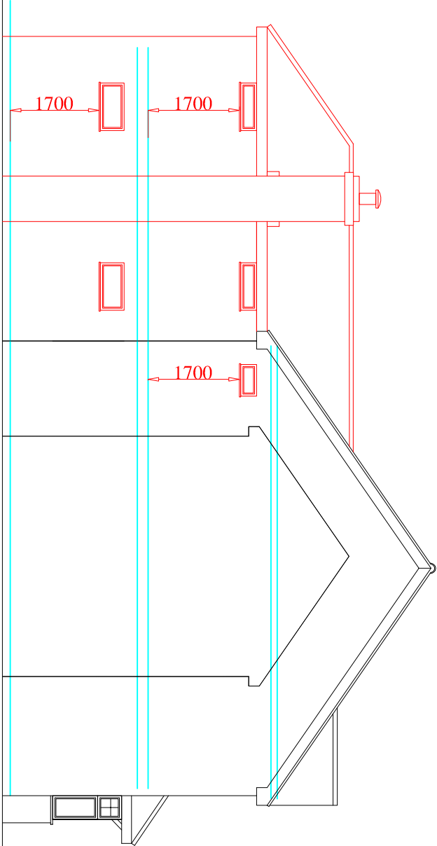
Proposed Side Elevation (south)
