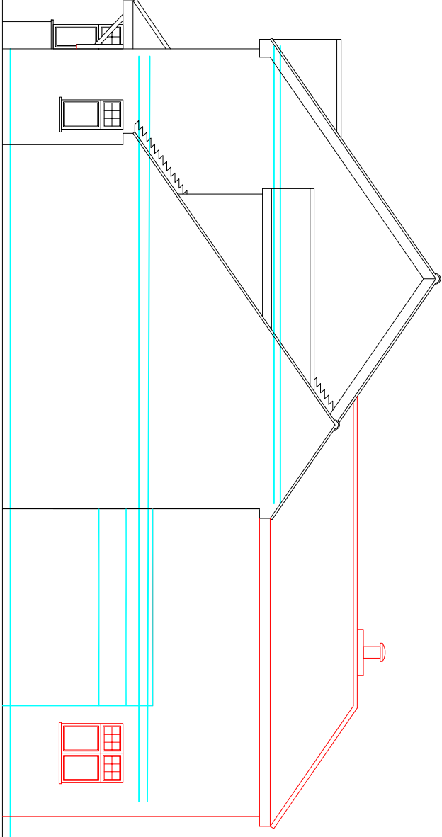
Proposed Side Elevation (north)
