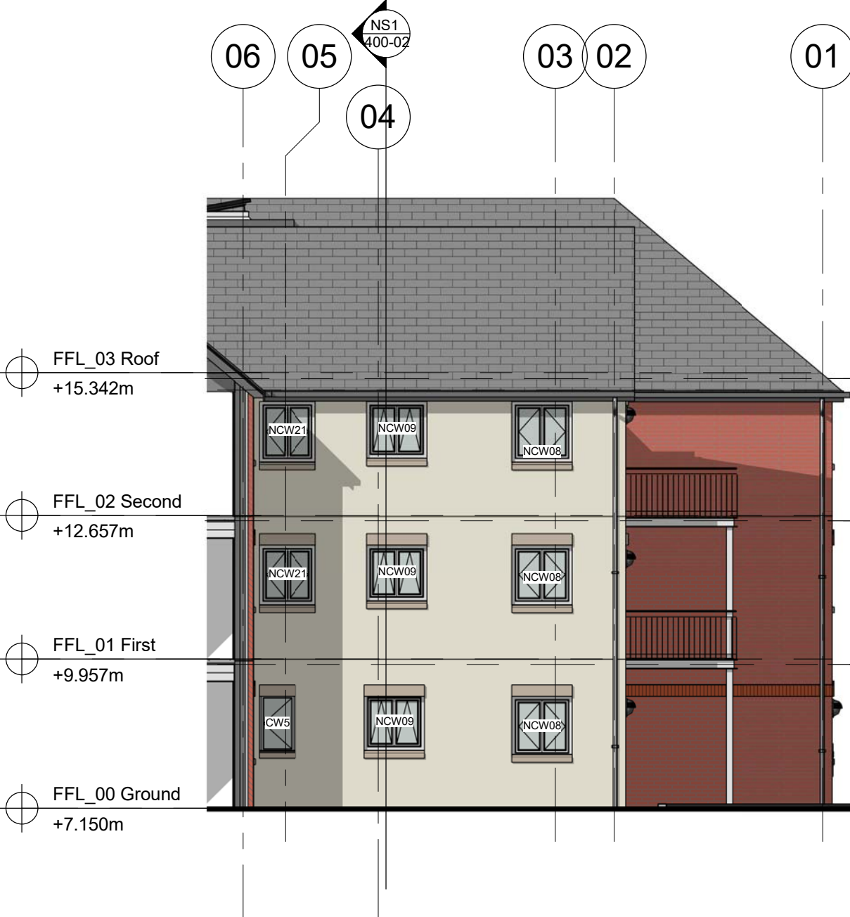
NORTH 1: 100
