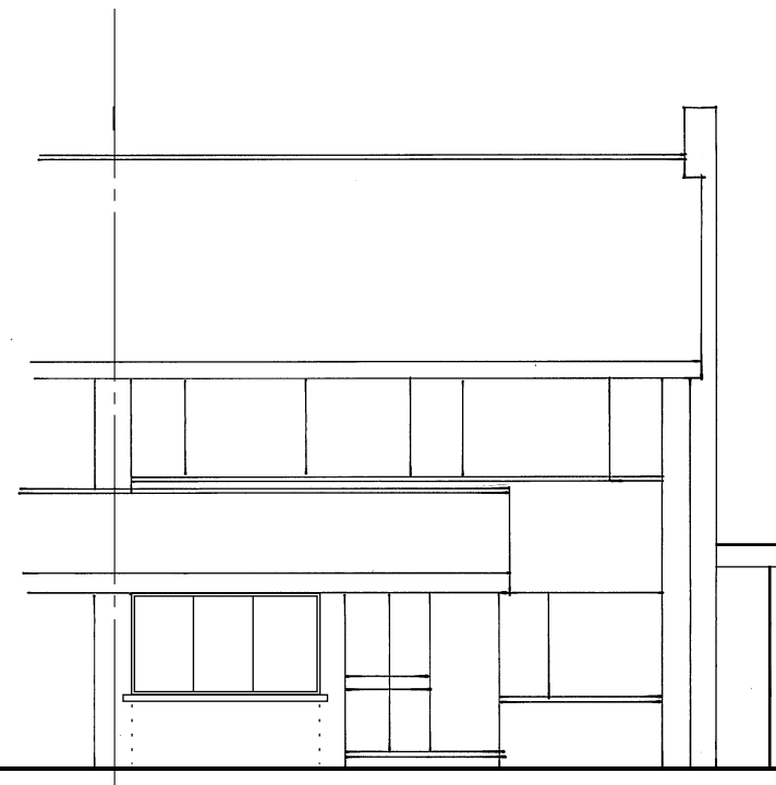
Proposed South/Front Elevation
