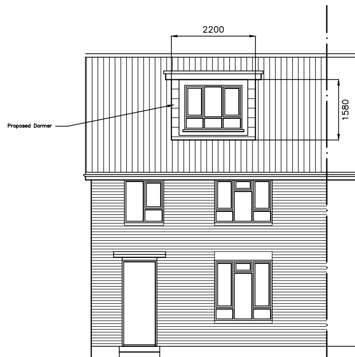
North Elevation
