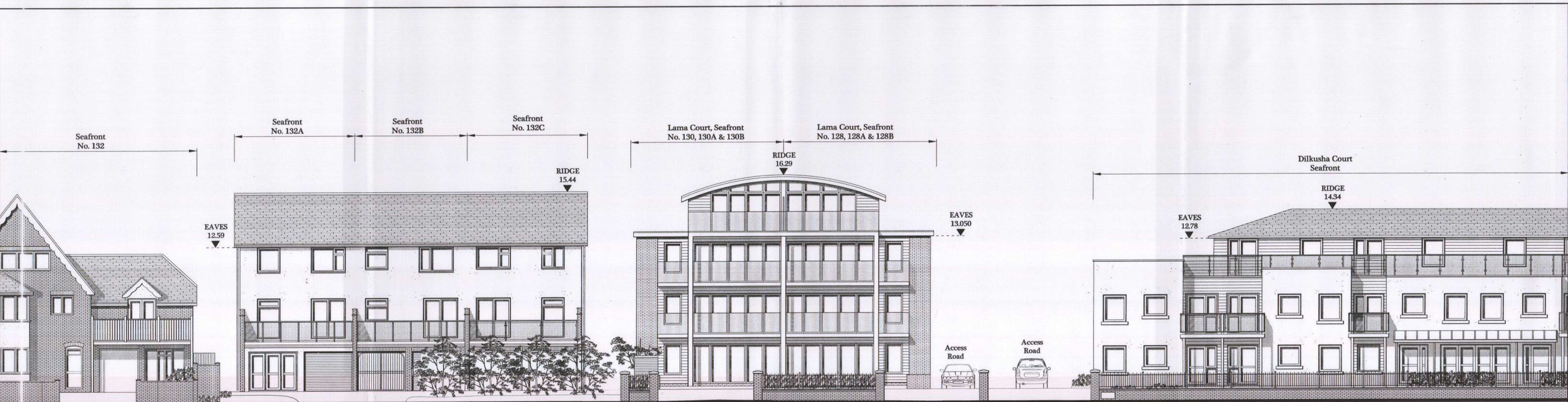
Proposed Street Elevation @ 1:100
