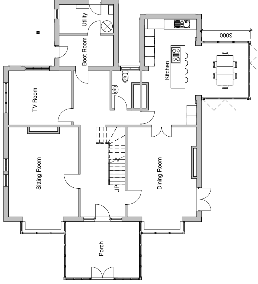
Proposed Ground Floor 1 : 100
