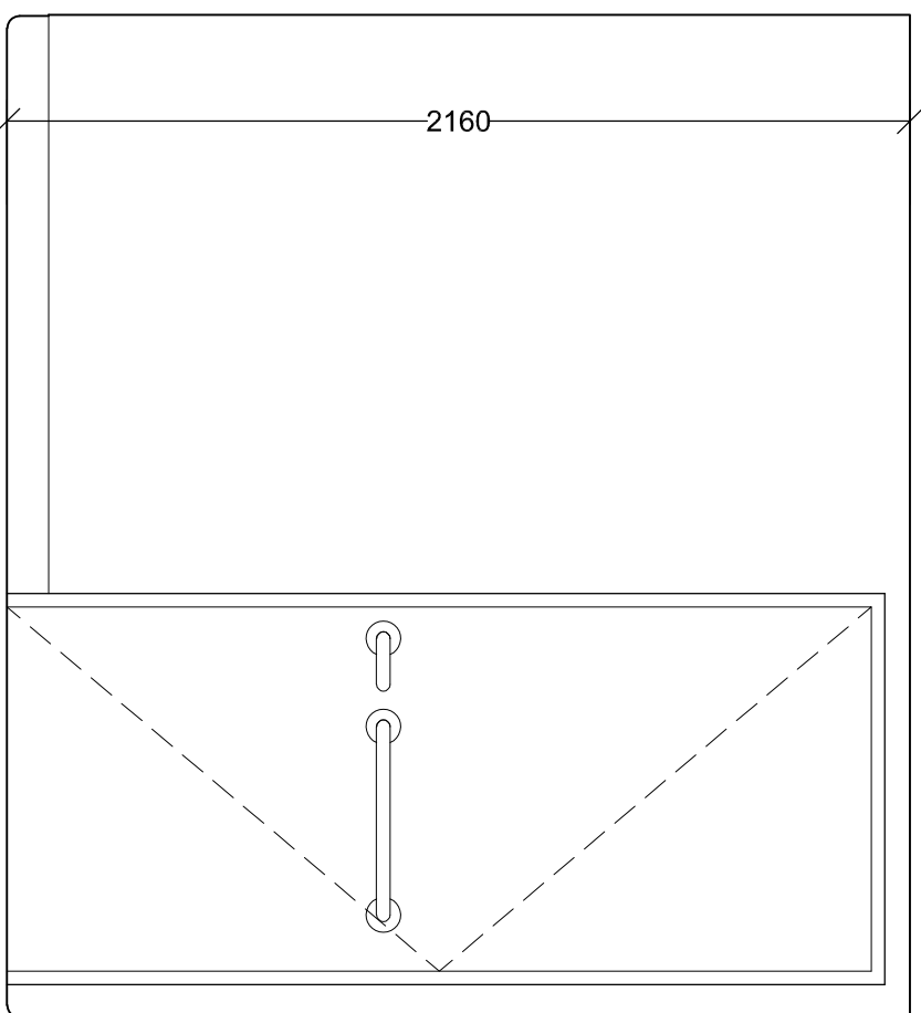
Elevation C
