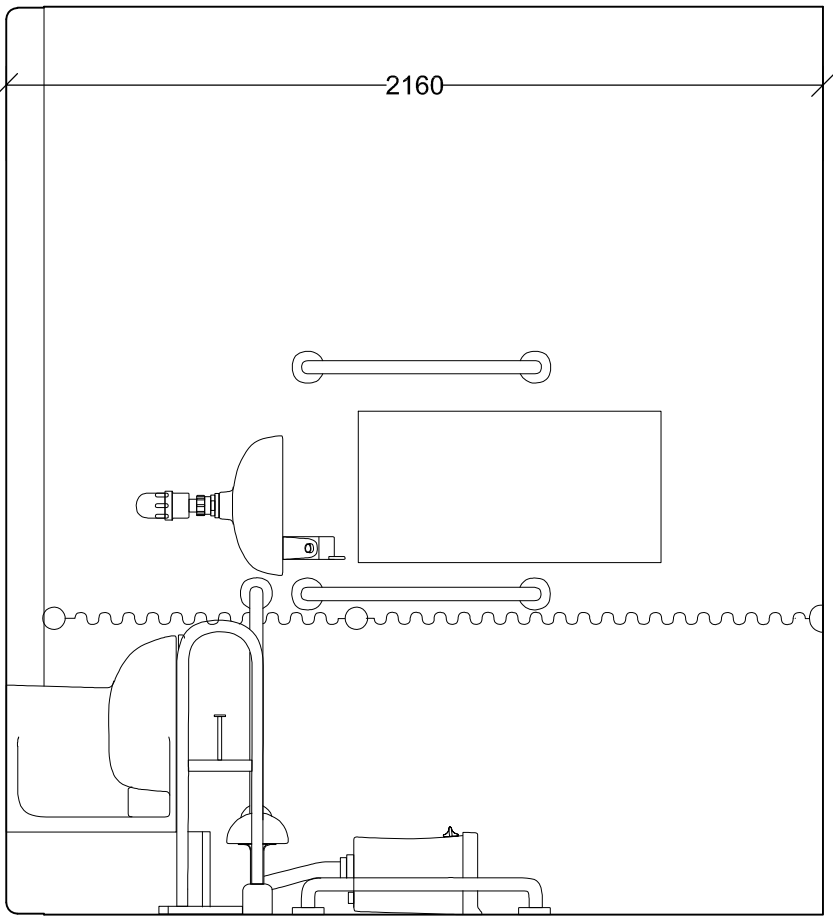
Elevation A Internal room elevations Scale 1:20
