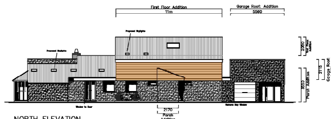
NORTH ELEVATION
