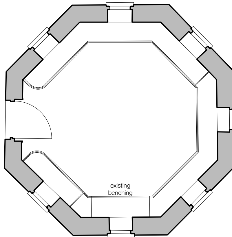
1 Dairy - Existing/Proposed Plan Scale: 1:50
