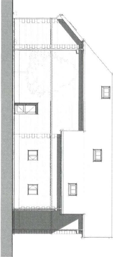
Rear Elevation 1 : 100
